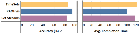
Figure 3: Overall accuracy and completion time of the three compared visualization techniques.
